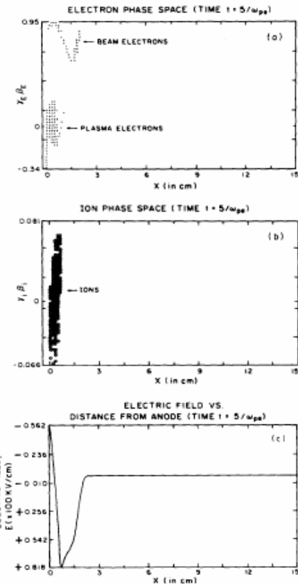
FIG. 3. Simulation phase space at early time t = 5/\omega_{pe} . (a) Electron phase space (beam and plasma), (b) ion phase space, (c) electron field versus position.
