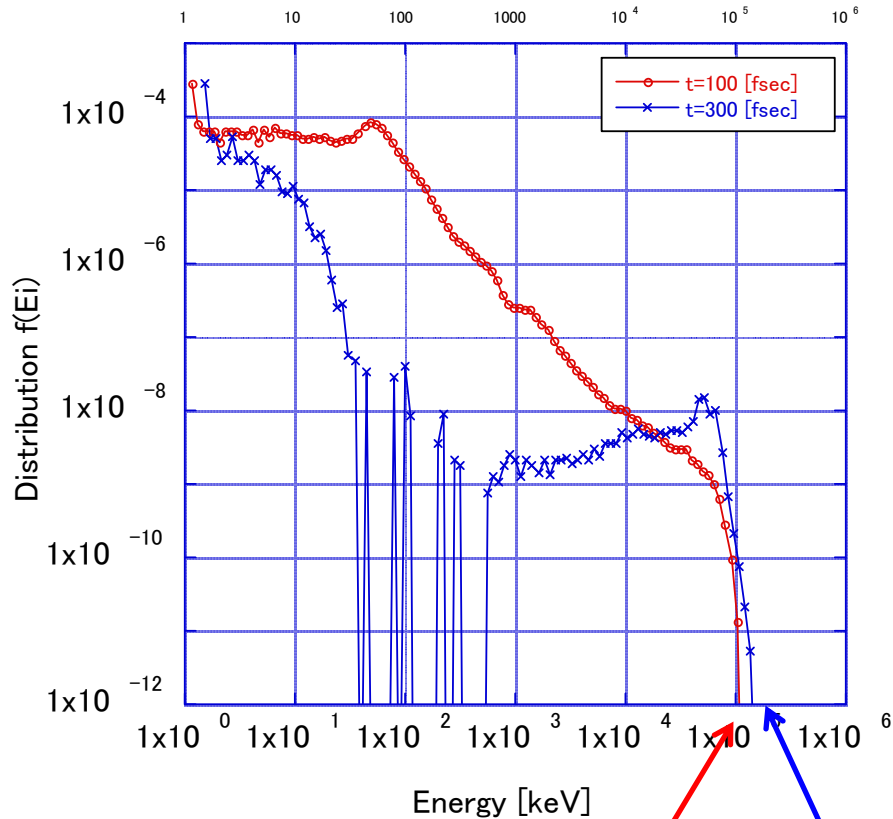
Ion Energy Distribution fEilog_a4_I820_Nxy128_p1m_r125nm Energy [keV]
