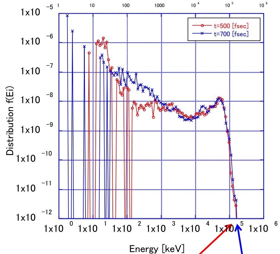
Ion Energy Distribution fEilog_a4_I820_Nxy128_p1m Energy [keV]
